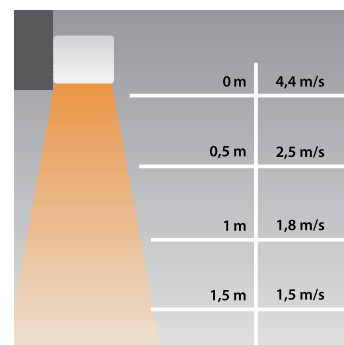
Air distance/speed COR-S
